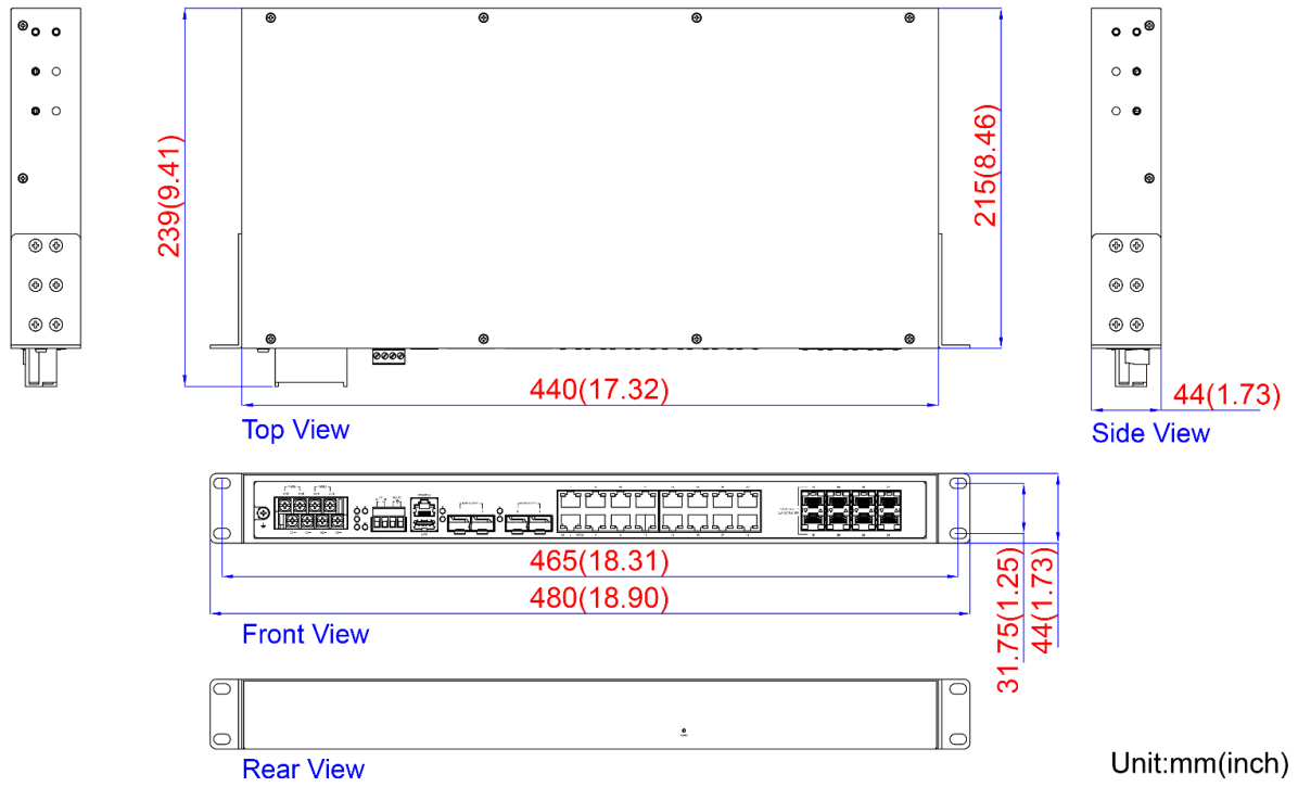
Figure 2.1 - Physical Dimensions
